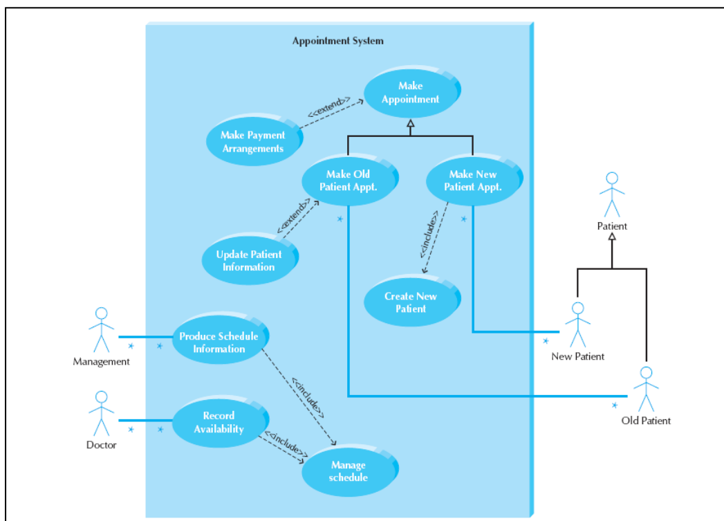
Use Case Diagram ( MAIN )
